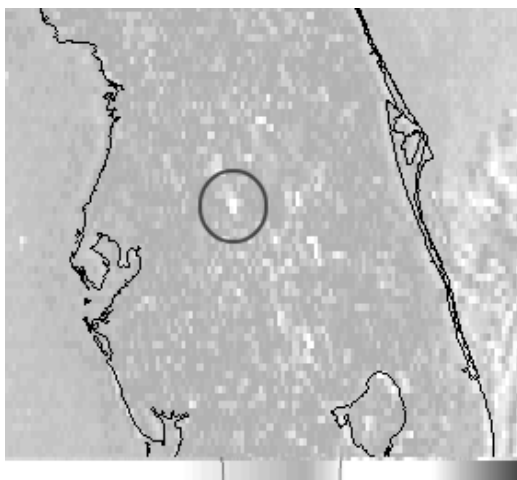
FIGURE 10 GOES-12 FOG/STRATUS PRODUCT 1015 UTC JANUARY 9, 2008
