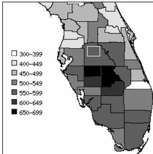
FIGURE 3 KEETCH BYRAM DROUGHT INDEX (KBDI) JANUARY 8, 2008
