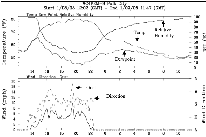
FIGURE 7 METEOGRAM FROM WC4PEM-9 POLK CITY, FLORIDA (28.19650, -81.78567, 36.8M), APPROXIMATELY 4 KM FROM CRASH SITE (MESOWEST)
