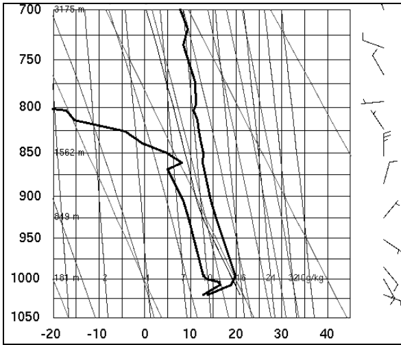
FIGURE 6 SKEW-T, VERTICAL PROFILE OF THE ATMOSPHERE TO 3175 M, RUSKIN, FLORIDA (TRUNCATED SKEW-T DIAGRAM), 1200 UTC, JANUARY 9, 2008 (LEFT TO RIGHT: DEWPOINT, TEMPERATURE, WIND BARBS IN KNOTS)
