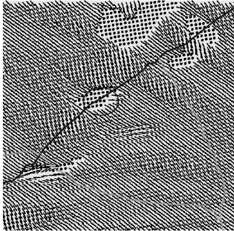
FIGURE 11 HIGH RESOLUTION (100 M) WRF 2 M WINDS (CIRCLE INDICATES ACCIDENT AREA)
