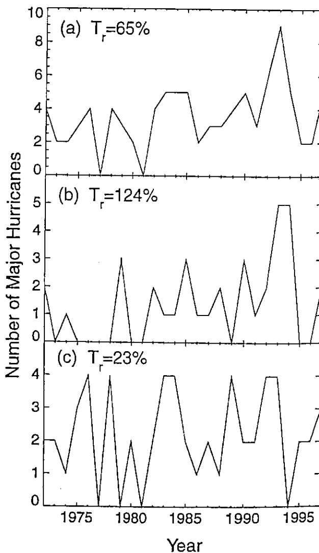
Figure 2. Time series of seasonal major hurricane numbers for the three regions, (a) Whole NE Pacific (b) Western and (c) Eastern, 1972-1997.
